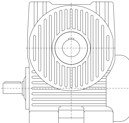
蜗轮蜗杆齿轮箱 Worm Gear Units
