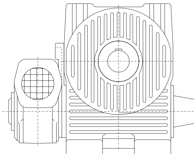
双级蜗轮蜗杆齿轮箱 Double Worm Gear Units
