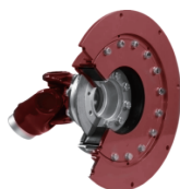
Couplings with cardan shaft 盘式高弹联轴器
